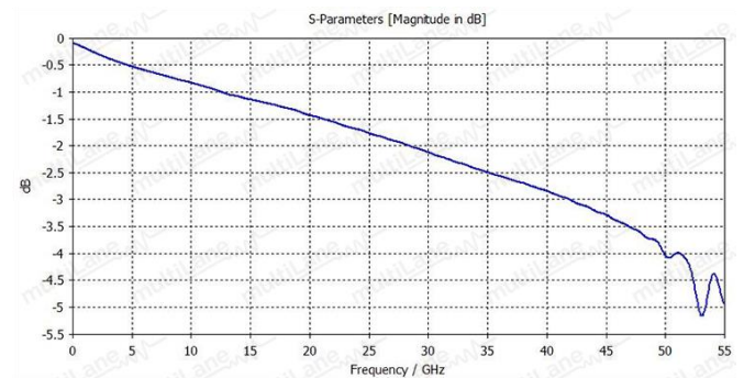
Figure 3: ML4020-112 Insertion Loss
